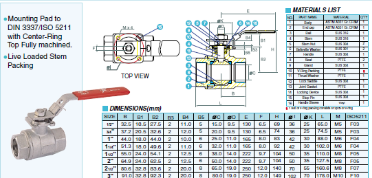
FIG. 20-50 FULL PORT 1/2" TO 3" 1000 PSI
