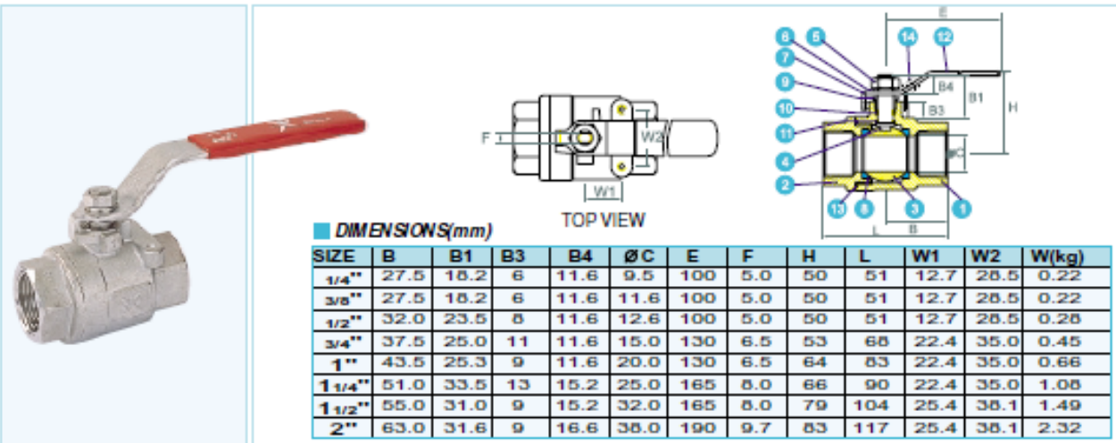
FIG. 20-40 FULL PORT 1/4" TO 1" 2000 PSI 1 1/4" TO 2" 1500 PSI
